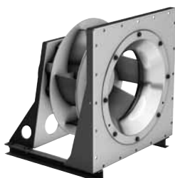
RLE E6-3540-EC-06/M6 36 kg
